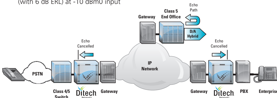
Ditech's HEC Solution for VoIP-PSTN Gateways
